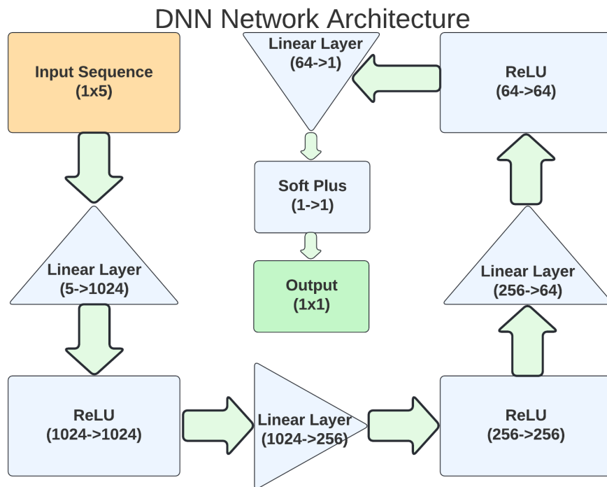
Figure 3.1: Diagram illustrating this study's LSTM (top) and RNN (bottom) architectures
