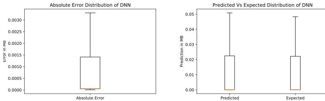
Figure 4.2: DNN on dataset 1, absolute error distribution (left) and predicted v. expected distribution (right)
