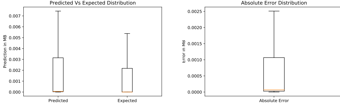
Figure 3.2: Box and whisker plots comparing the distributions of predicted and expected data (left), and a box and whisker plot of the distribution of error (right)
