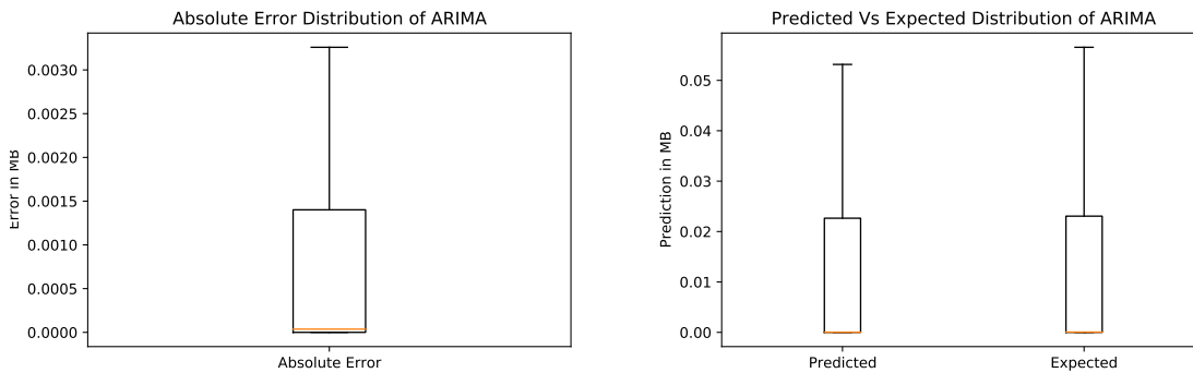
Figure 4.1: ARIMA on dataset 1, absolute error distribution (left) and predicted v. expected distribution (right)
