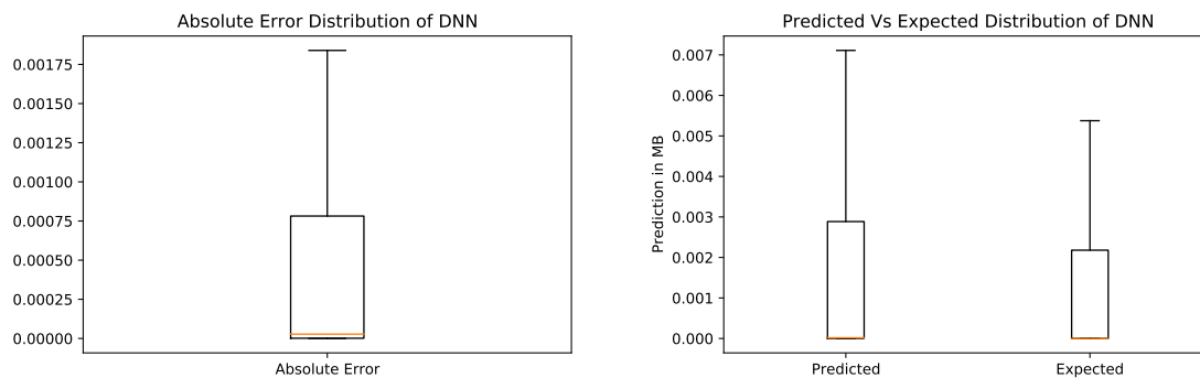
Figure 4.5: DNN on dataset 2, absolute error distribution (left) and predicted v. expected distribution (right)
