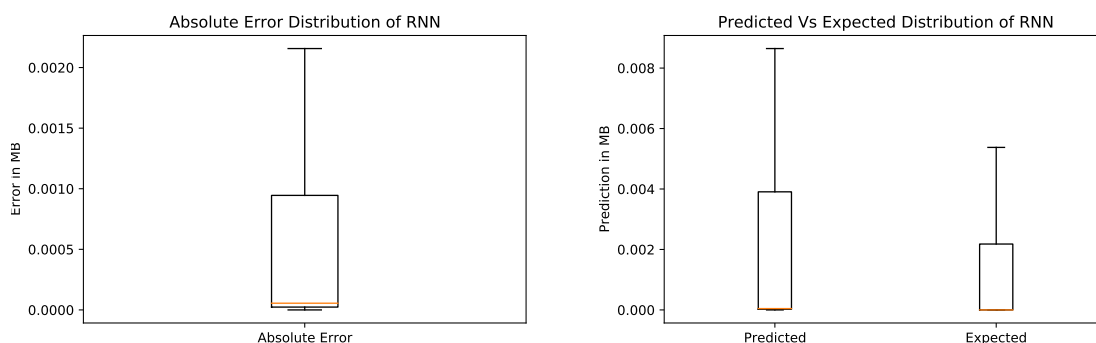
Figure 4.6: RNN on dataset 2, absolute error distribution (left) and predicted v. expected distribution (right)
