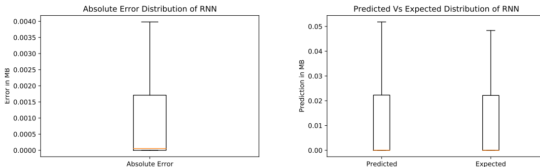
Figure 4.3: RNN on dataset 1, absolute error distribution (left) and predicted v. expected distribution (right)
