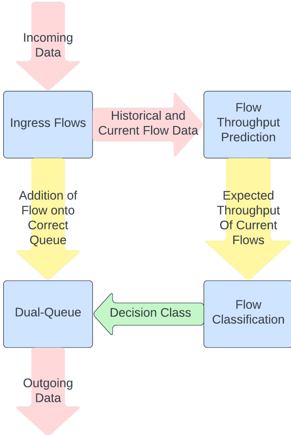
Figure 1.1: Diagram illustrating the general structure of Dual-Queue AQM and the flow of data through it with respect to the work of this study
