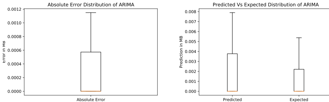
Figure 4.4: ARIMA on dataset 2, absolute error distribution (left) and predicted v. expected distribution (right)
