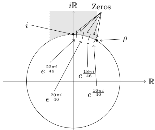
Figure 1.3.2: The five zeros of E_{46}
