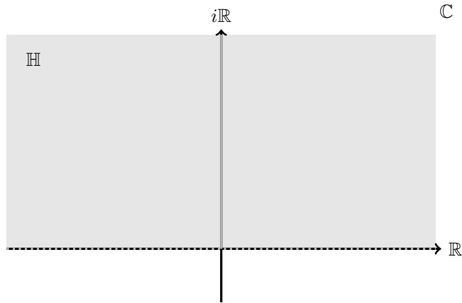
Figure 1.1.1: The Upper Half Plane
