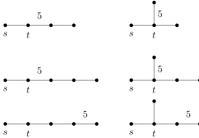
FIGURE 4. The last remaining obstructions to Theorem 7.1.
