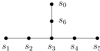
FIGURE 1. The Coxeter graph of type \tilde{E}_6 .
