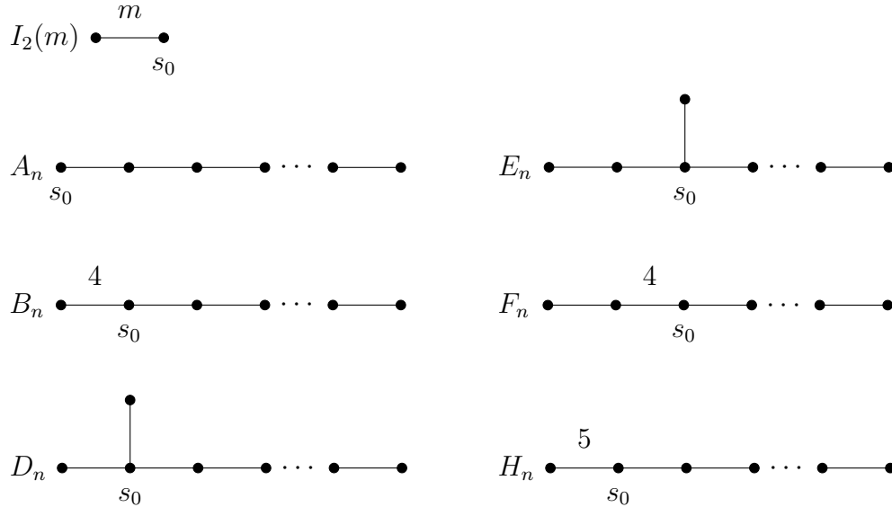
FIGURE 3. Connected Coxeter graphs corresponding to CFC-finite groups.
