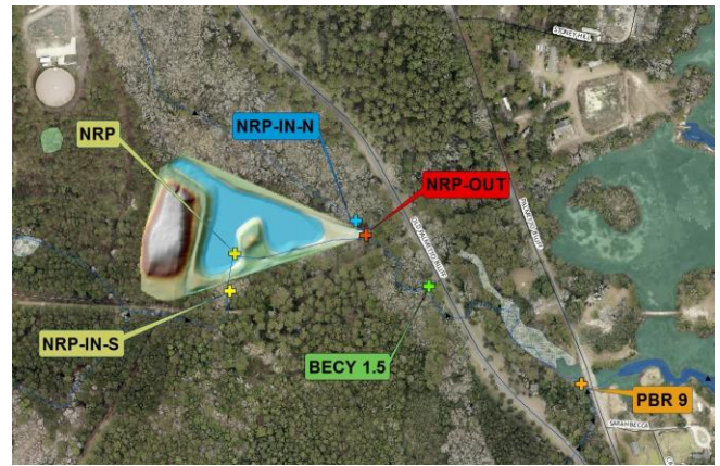
Figure 1 - New Riverside BMP Sampling Locations
