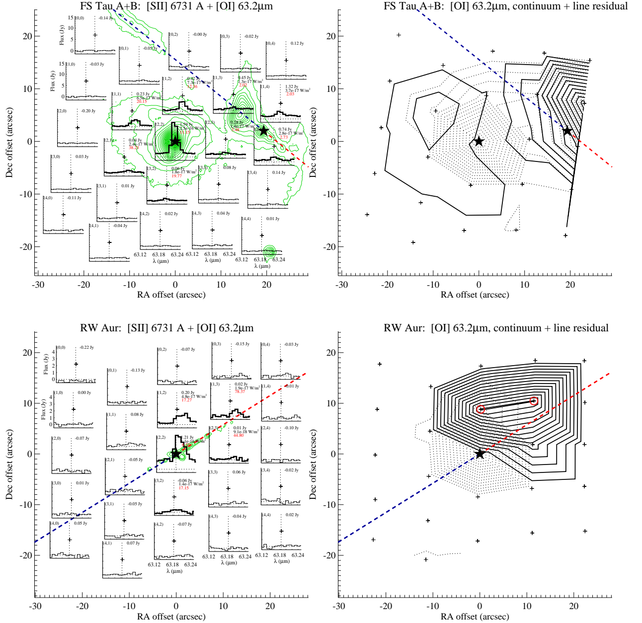
Fig. 2. Left panel: [O I] 63 \mu\text{m} line spectra in the 25 spaxels of the PACS array. Each spaxel is labelled by its (x,y) index and its position is indicated by a black cross. The RA and Declination offsets with respect to the source (in arcseconds) are indicated on the x and y axis. The black star is the source position and the blue/red dashed lines the position angle of the optical-jet blue/red lobe. In each spectrum, vertical and horizontal dotted lines show the line wavelength and the zero flux level, respectively. In those spaxels where the line is detected above the 3\sigma level, the spectrum is drawn with a black thick line, and the estimated continuum level (in Jy), line flux (in \text{W m}^{-2} ), and line-to-continuum ratio (in red) are indicated. Where the line is not detected only the estimated continuum level (in Jy) is given. The optical-jet emission in the [S II] \lambda\lambda 6716, 6731 \text{ \AA} forbidden lines is overplotted (green contours). Contours are from Solf & Böhm (1999) (T Tau), Eisloffel & Mundt (1998) (DG Tau A, DG Tau B, FS Tau A+B), and Dougados et al. (2000) (RW Aur). Right panel: Contour levels of continuum (dotted lines) and line residual (solid lines) emission obtained from the analysis in Appendix B. The spaxels where residual line emission is detected with a confidence level \geq 5 are highlighted by a red circle (for RW Aur the red circles indicate residual emission above the 2\sigma level). The contours indicate that the line emission is shifted and/or more extended with respect to the continuum emission along the optical jet PA.
