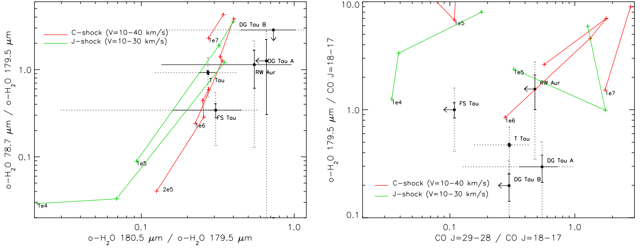
Fig. 6. Observed \text{H}_2\text{O} and CO line ratios (black dots) are compared with the predictions of slow C-type (red lines) and J-type (green lines) shock models (Flower & Pineau Des Forêts 2010). The solid lines indicate the errors due to the line signal-to-noise, while the dashed lines indicate the total error, obtained by adding the 30% error in the PACS flux calibration. The crosses along the red and green curves correspond to increasing shock velocity, from 10 \text{ km s}^{-1} to 40 \text{ km s}^{-1} (C-type shocks) or from 10 \text{ km s}^{-1} to 30 \text{ km s}^{-1} (J-type shocks). At the lowest velocity ( V_{\text{shock}} = 10 \text{ km s}^{-1} ), the pre-shock density is given.
