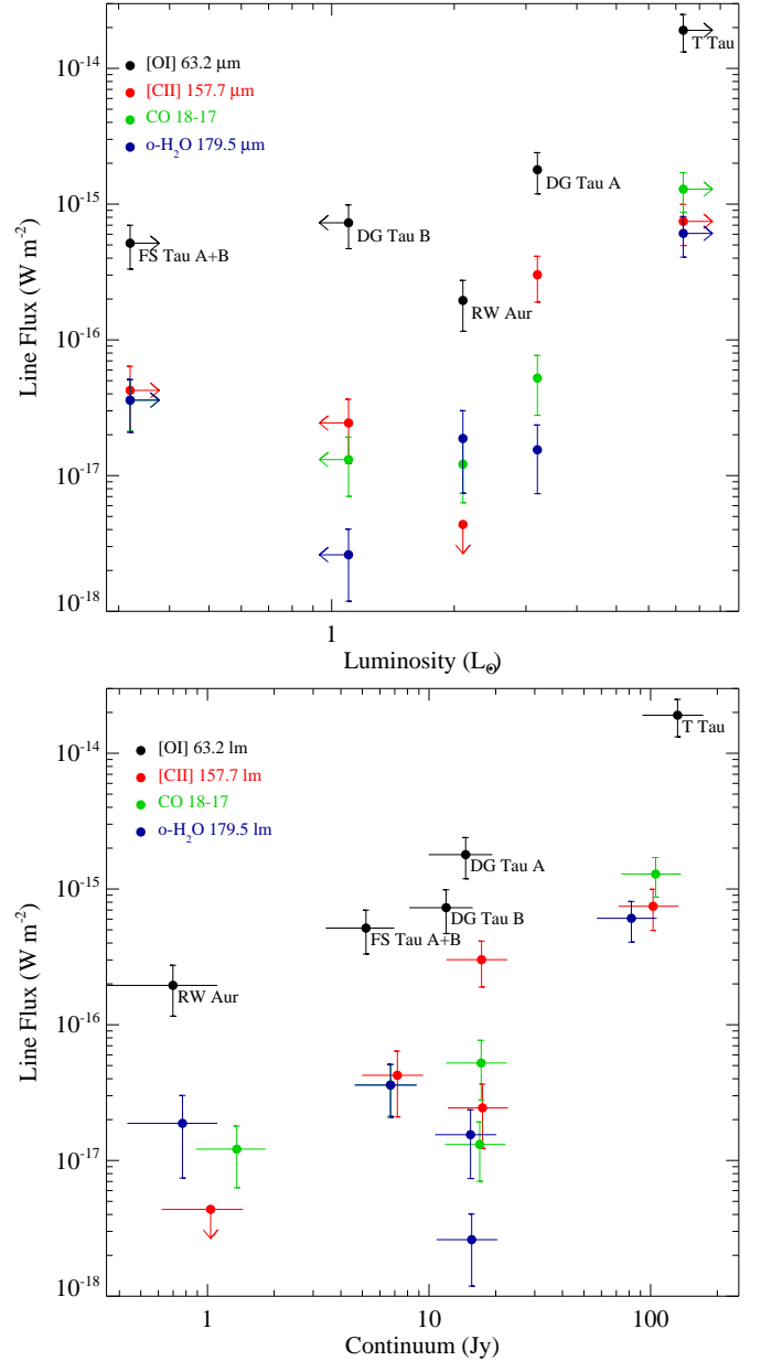
Fig. 3. The fluxes of the [O I] 63 \mu\text{m} , the [C II] 158 \mu\text{m} , the CO J=18-17, and the o- \text{H}_2\text{O} 179.5 \mu\text{m} lines are plotted versus the source luminosity ( left panel ) and their adjacent continuum ( right panel ) for all the sources in our sample (black, red, green, and blue dots). For FS Tau A+B and T Tau N+S the plotted source luminosity is a lower limit, since L_* of the Class I components FS Tau B and T Tau S is unknown. The upper limit on the stellar luminosity for DG Tau B corresponds to its bolometric luminosity as estimated by Kruger et al. (2011).
