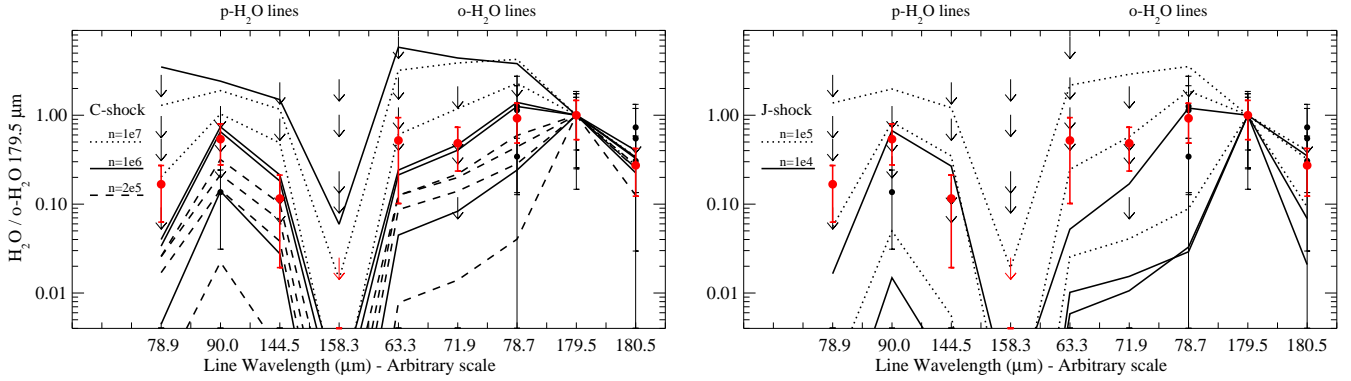
Fig. 7. Observed \text{H}_2\text{O} line ratios for T Tau (red points/arrows) are compared with the predictions of C-type (left panel) and J-type (right panel) shock models (Flower & Pineau Des Forêts 2010) with relatively high pre-shock densities. The \text{H}_2\text{O} line ratios and upper limits for the other sources in the sample are overplotted (black points and arrows).
