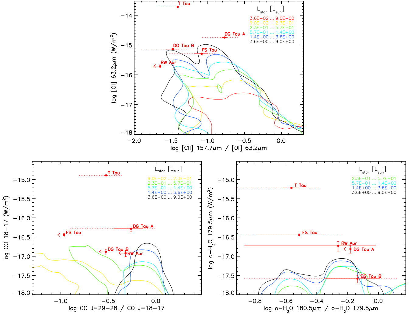
Fig. 4. Observed [O I], [C II], CO, and H 2 O line fluxes and ratios (red dots) are compared with predictions from a subsample of disk models from the DENT grid (Woitke et al. 2010; Kamp et al. 2011). Contours encircle 85% of the DENT disks for star luminosity values from 10^{-2} L_{\odot} to 9 L_{\odot} (red, yellow, green, cyan, blue, and black crosses). The total errors on the observed values (dotted red lines) are obtained summing the error due to the line signal-to-noise (solid red lines) and the 30% error affecting PACS flux calibration. The subsample of disk models is obtained by selecting M \leq 2.5 M_{\odot} , T_{eff} \leq 5500 K, L \leq 9 L_{\odot} , R_{in} = R_{subl} , and dust-to-gas ratio = 0.01.
