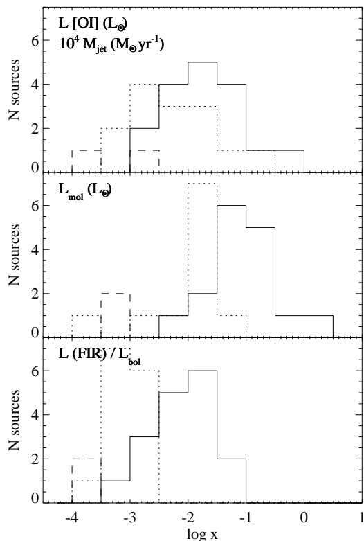
Fig. 9. Histograms of L [O I] ( upper panel ), L_{mol} ( middle panel ), and L (FIR)/ L_{bol} ( bottom panel ) for Class 0, I, and II sources (solid, dotted, and dashed lines).
