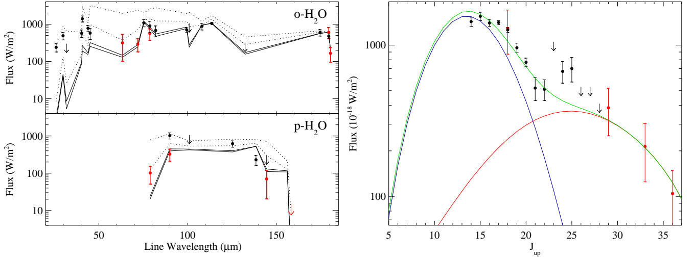
Fig. 8. All the available ISO (black points) and Herschel (red points) observations of H 2 O ( left panel ) and CO ( right panel ) lines for T Tau are shown. Left panel: Line fluxes predicted by a slow C-shock for an emitting area of \sim 360 AU diameter and pre-shock density of n=10^6 cm -3 (velocity V=20 - 30 km s -1 , dotted lines), or n=10^7 cm -3 ( V=10 - 20 km s -1 , dotted lines). The low-excitation water lines are well reproduced by C-shock with pre-shock density of 10^6 cm -3 while the higher excitation lines require higher pre-shock density. Right panel: CO line fluxes predicted by: a C-shock model ( n=10^6 cm -3 , V=20 - 30 km s -1 , emitting area diameter, D=360 AU, red line ); an LVG warm gas component ( n=10^6 , T=300 K, D=360 AU, N_{CO}=1.5 \cdot 10^{18} cm -2 , blue line ); the sum of the two models ( green line ). While the high- J CO lines are well reproduced by the same C-shock model used for water lines, a warm gas component is required to simultaneously fit the lower- J lines observed with ISO (down to J_{up}=14 ).
