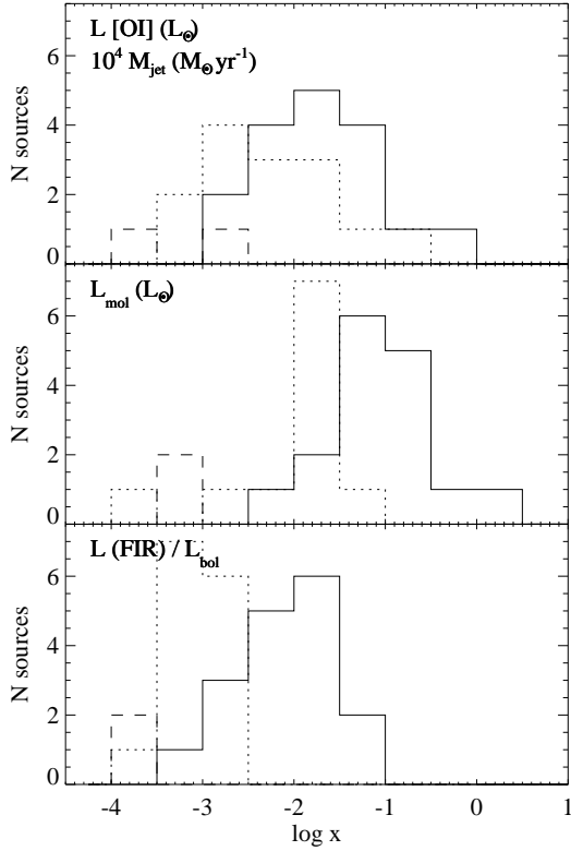
Fig. 9. Histograms of L[\text{OI}] (upper panel), L_{\text{mol}} (middle panel), and L(\text{FIR})/L_{\text{bol}} (bottom panel) for Class 0, I, and II sources (solid, dotted, and dashed lines).
