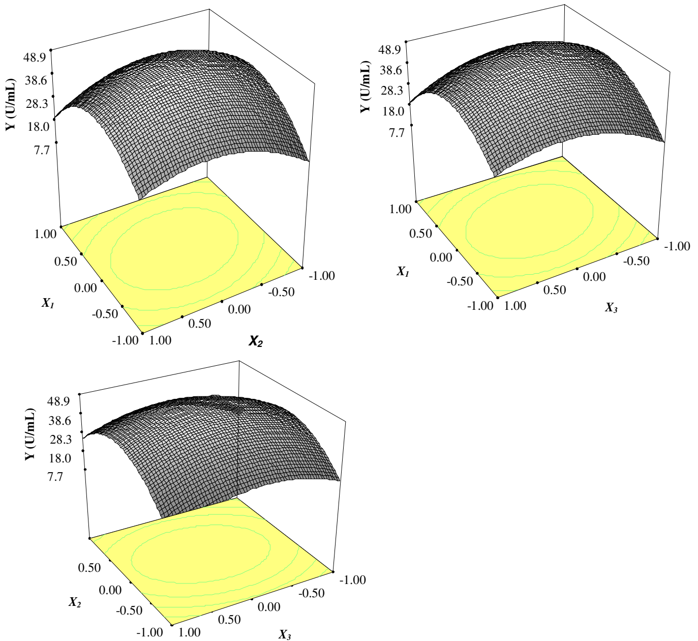
Figure 3. The response surface plots showing the influences of glucose ( X_1 ), corn steep flour ( X_2 ) and K_2HPO_4 ( X_3 ) against keratinase production ( Y ) by B. licheniformis ZJUJEL31410*. * X_1 was the coded value of glucose, X_2 was the coded value of corn steep flour, X_3 was the coded value of K_2HPO_4 , and Y was keratinase production.
