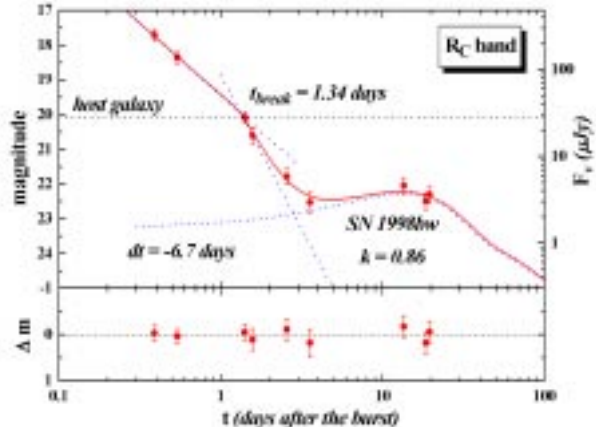
Fig. 12.— The same as Fig. 8 but with dt (eq. 2) as a further free parameter.
