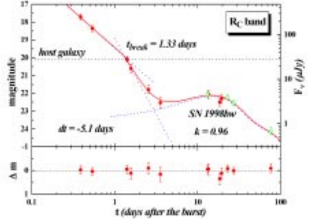
Fig. 14.— The same as Fig. 12 but with the inclusion of published HST R -band data from Bloom et al. (2002).
