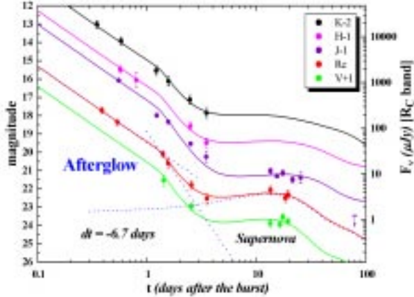
Fig. 13.— The same as Fig. 9 but for dt = -6.7 days.
