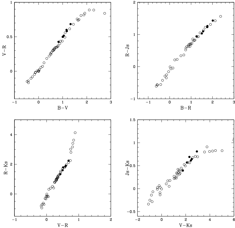
Fig. 5.— Color-color diagrams of bright, non-saturated stars detected in the central area of the images of GRB 011121 (filled circles), compared with the expected color-color sequence as derived from the convolution of the stellar library of Pickles with the total filter efficiency curves of the instruments used (open circles).
