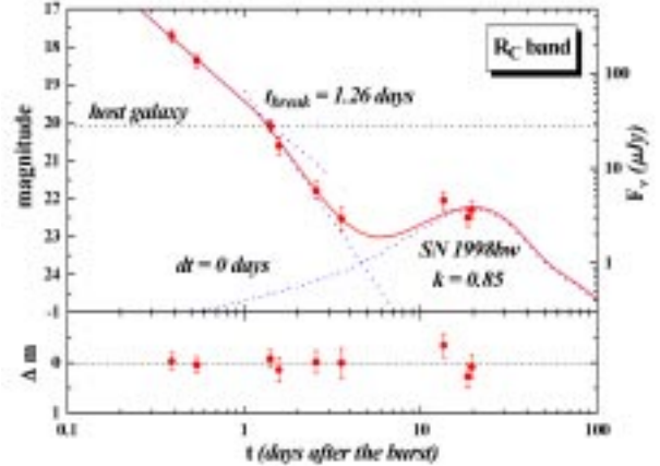
Fig. 8.— R_c -band light curve based on eq. (1) and an additional supernova component, assuming dt = 0 days (eq. 2). Note that all photometric data are corrected for Galactic extinction (§3.2). Compared to Tab. 1 a conservative systematic 1\sigma error of 0.15 mag has been added to all data.
