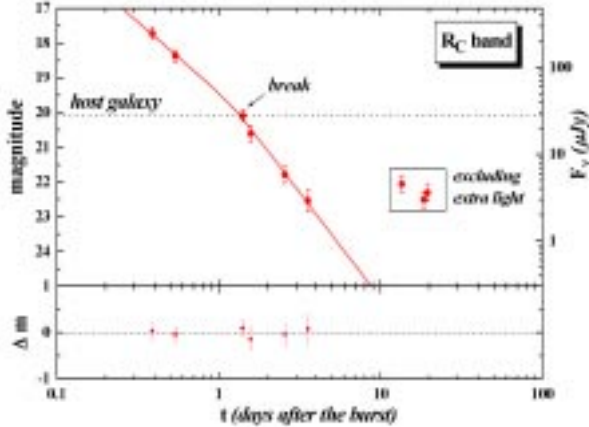
Fig. 7.— R_c -band light curve of the afterglow of GRB 01121 and a fit to the data prior to t = 10 days. Compared to Tab. 1 a conservative systematic 1\sigma error of 0.15 mag has been added to all data. The break in the power-law decay occurs at t_b = 1.2 days. At late times the afterglow is significantly brighter than predicted by the power-law. Note the particularly bright host galaxy.
